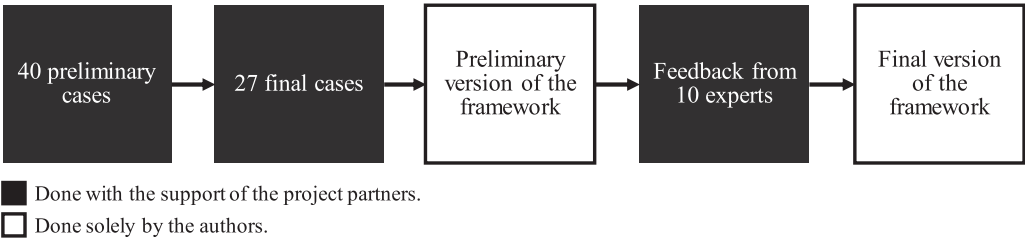
Figure 1. Methodological process.
